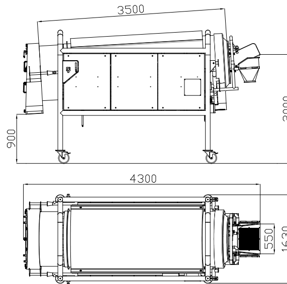
Drawings of the TUX 1000 model
